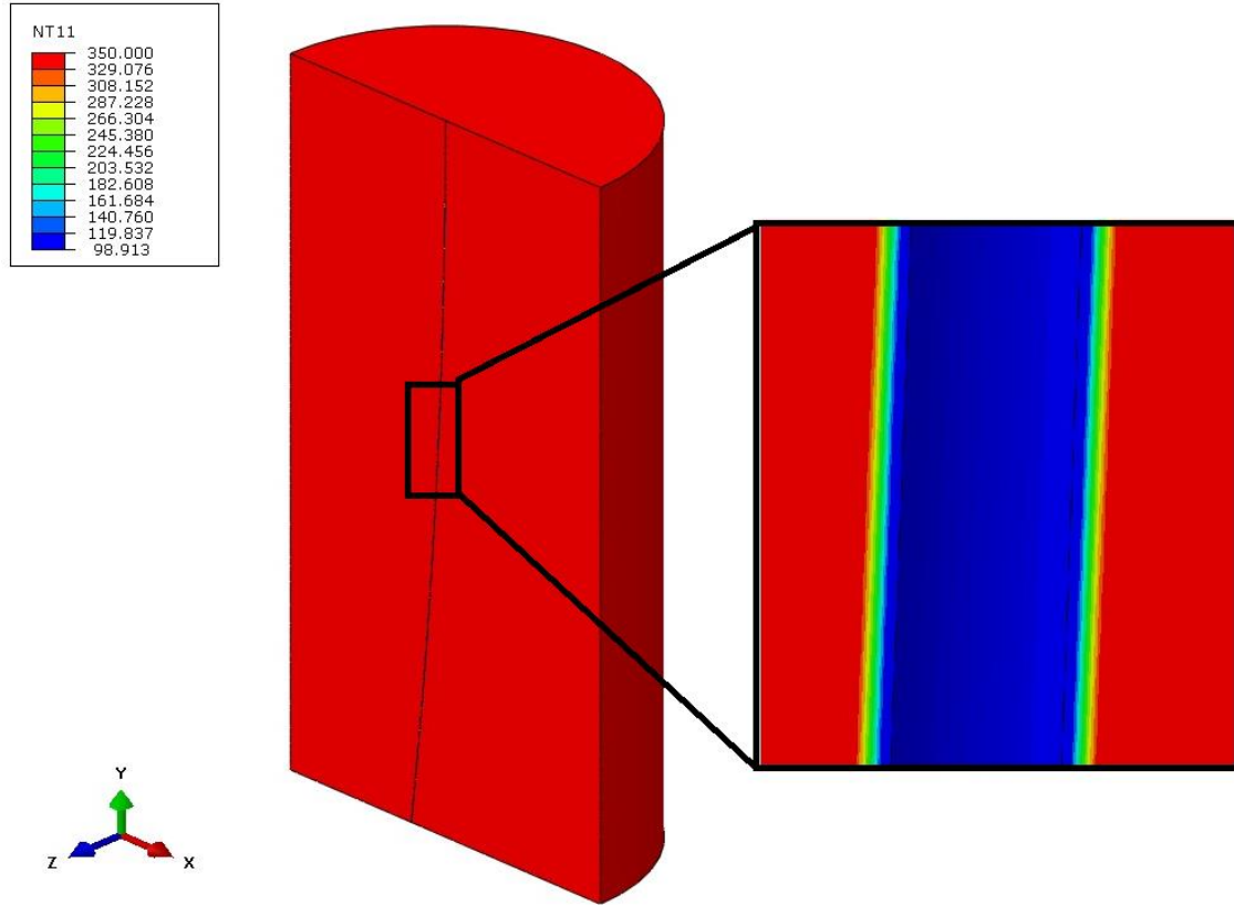
Figure 50 Heat transfer analysis results for deviated well
