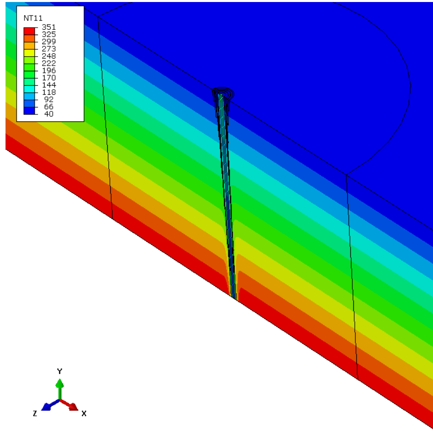
Figure 12 Global FE model – Well stimulation temperature profile
