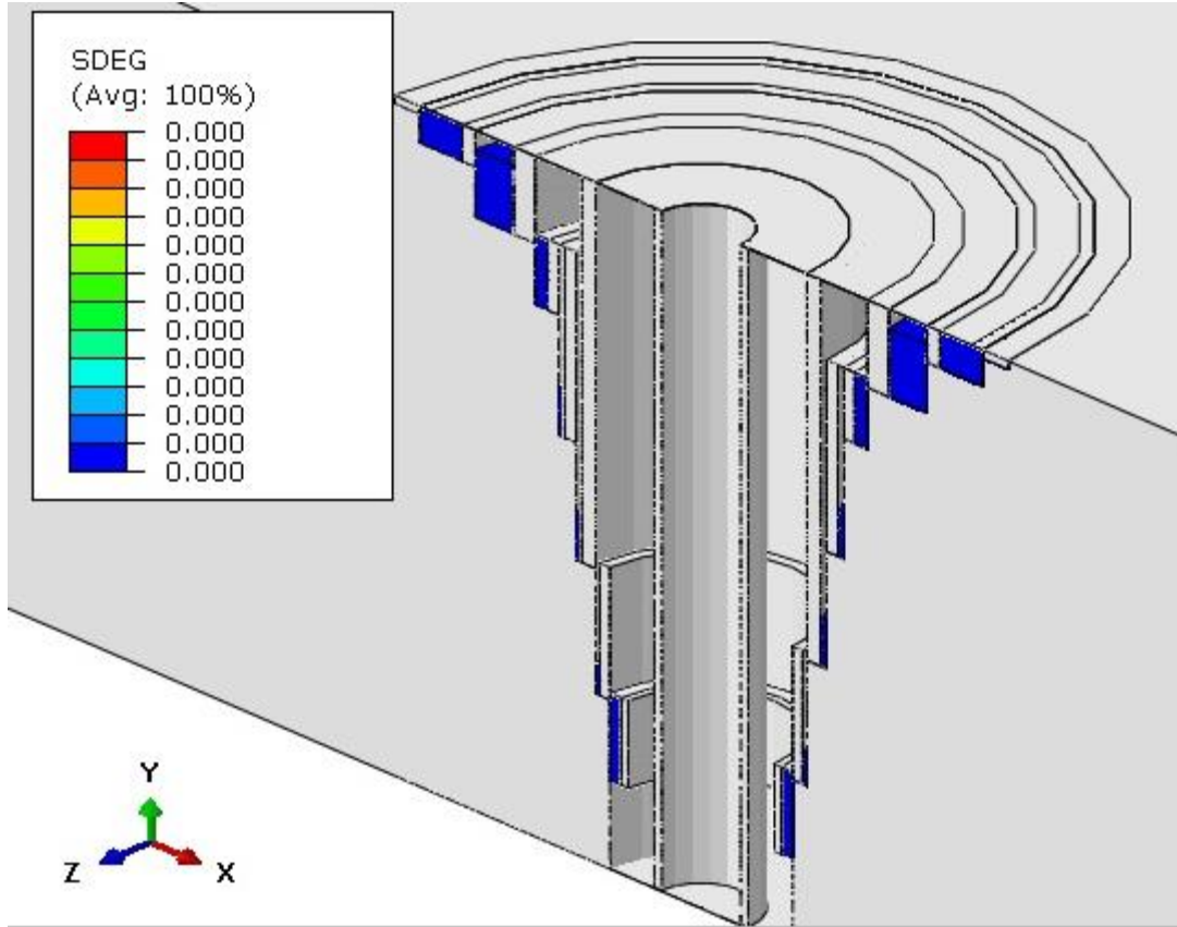
Figure 17 Cement damage after first year of cycles
