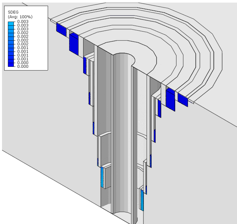
Figure 40 Cycle-4x-60-3207 Case cement damage after first stimulation
