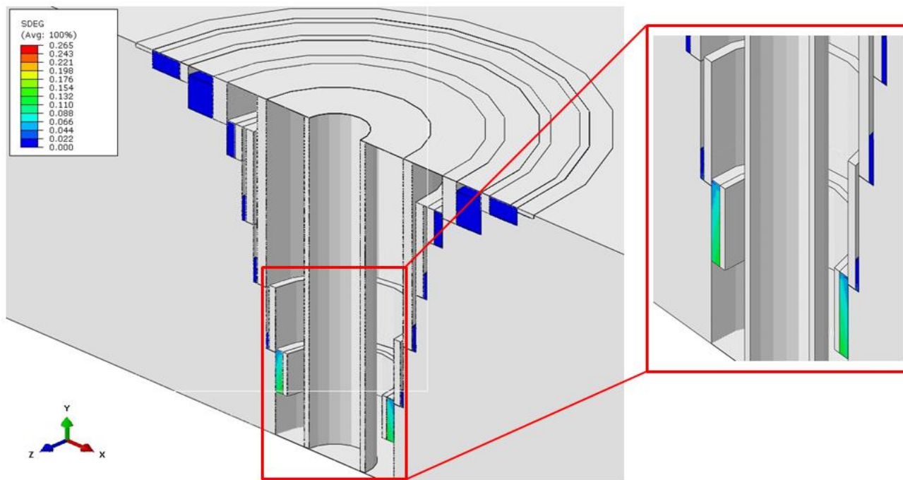
Figure 32 Cycle-4x-60-6310 Case cement damage after first stimulation
