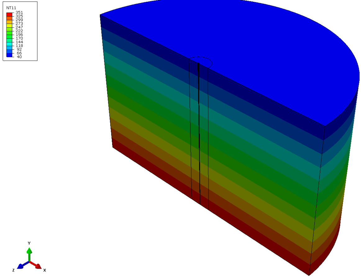
Global FE model – Initial temperature profile
