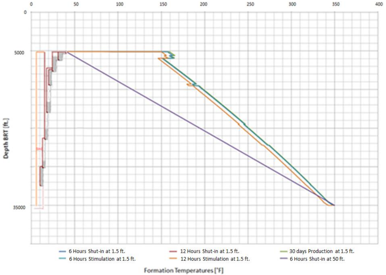
Figure 5 Temperature profile in formation near wellbore
