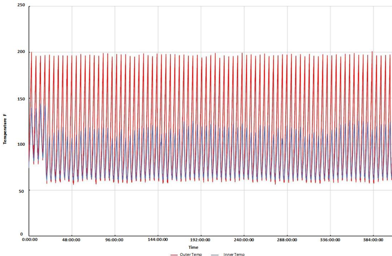
Figure 70 Thermal shock example – cycle history
