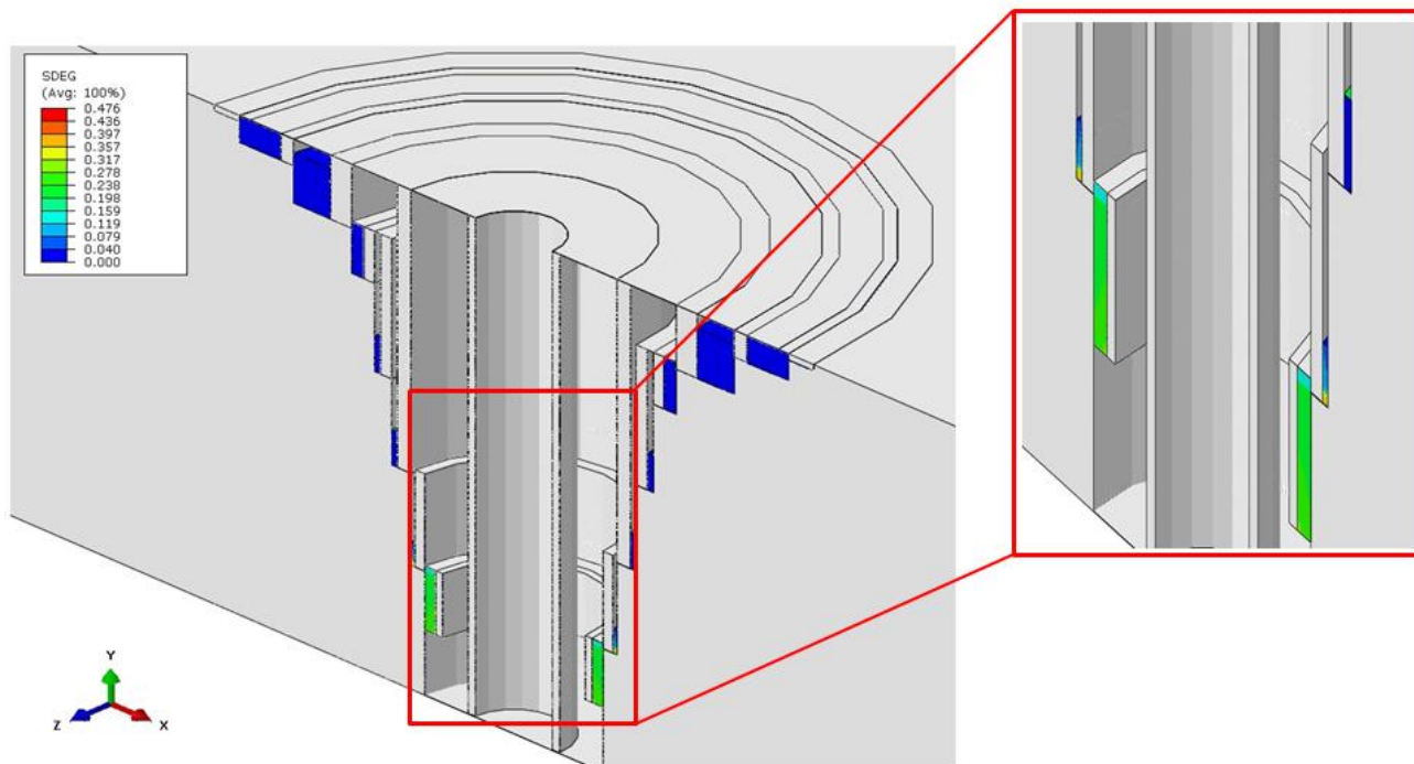
Figure 34 Cycle-4x-60-6310 Case cement damage after third stimulation
