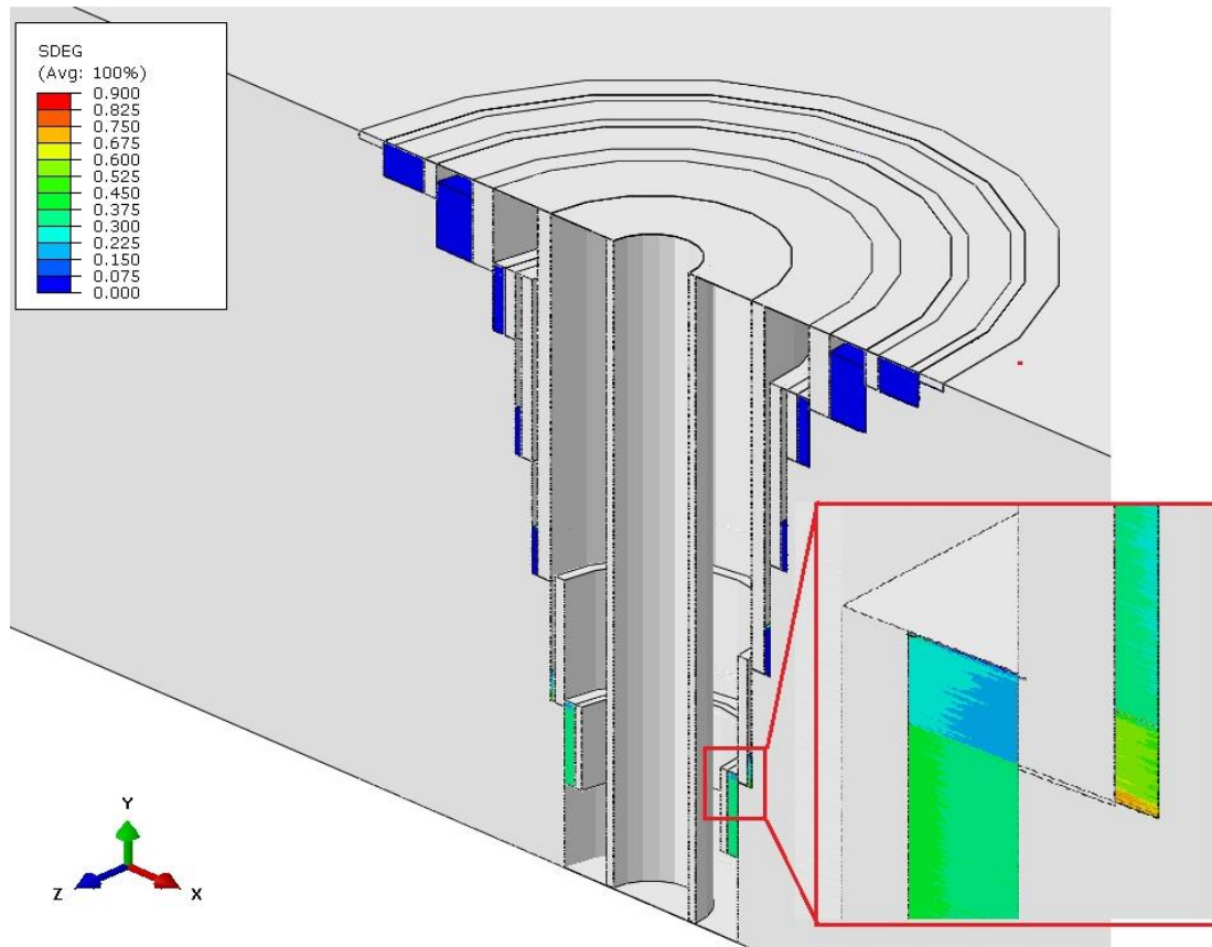
Figure 26 Cement damage after 20 years of cycles
