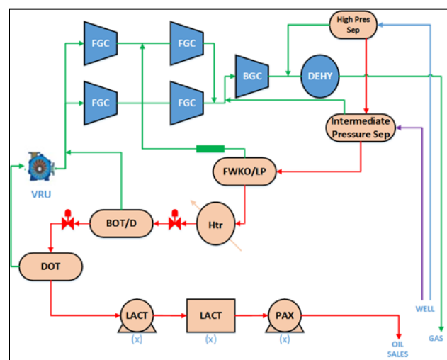
Exhibit 1: Typical Offshore Production Train 1
