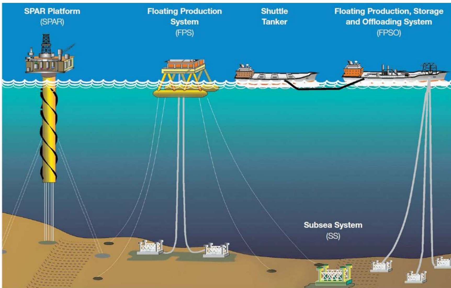
Figure 7: Typical Types of Platforms in Use on the OCS (2 of 2).
