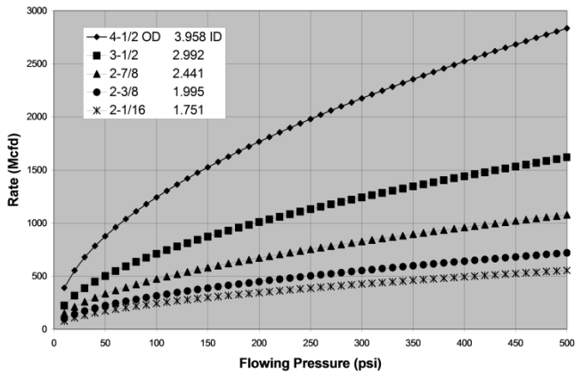
Exhibit 2: Schematic of the Turner Unloading Rate for Wells Producing Water 1
