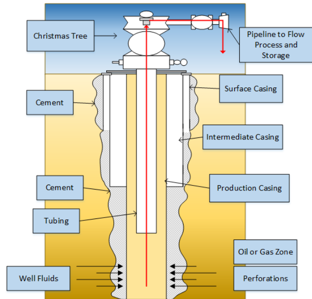
Exhibit 1: Tubing and/or Annular Flow Is Possible.
