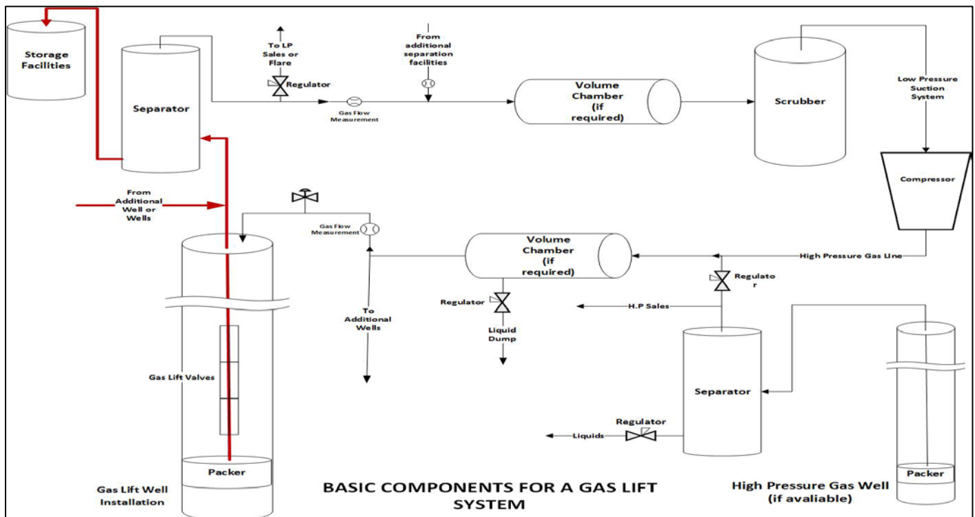
Exhibit 3: Typical Gas Lift System source: Argonne Vent/Flare Research Team
