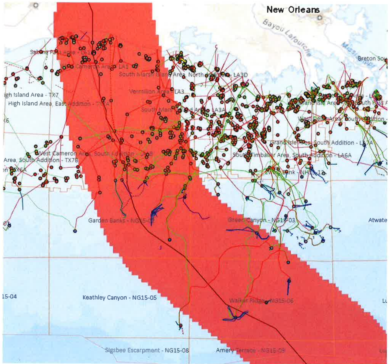
Figure 1: Hurricane Laura Affected Area [Area of Hurricane Force Winds is in Red - Plotted using information from NOAA – National Hurricane Center]
