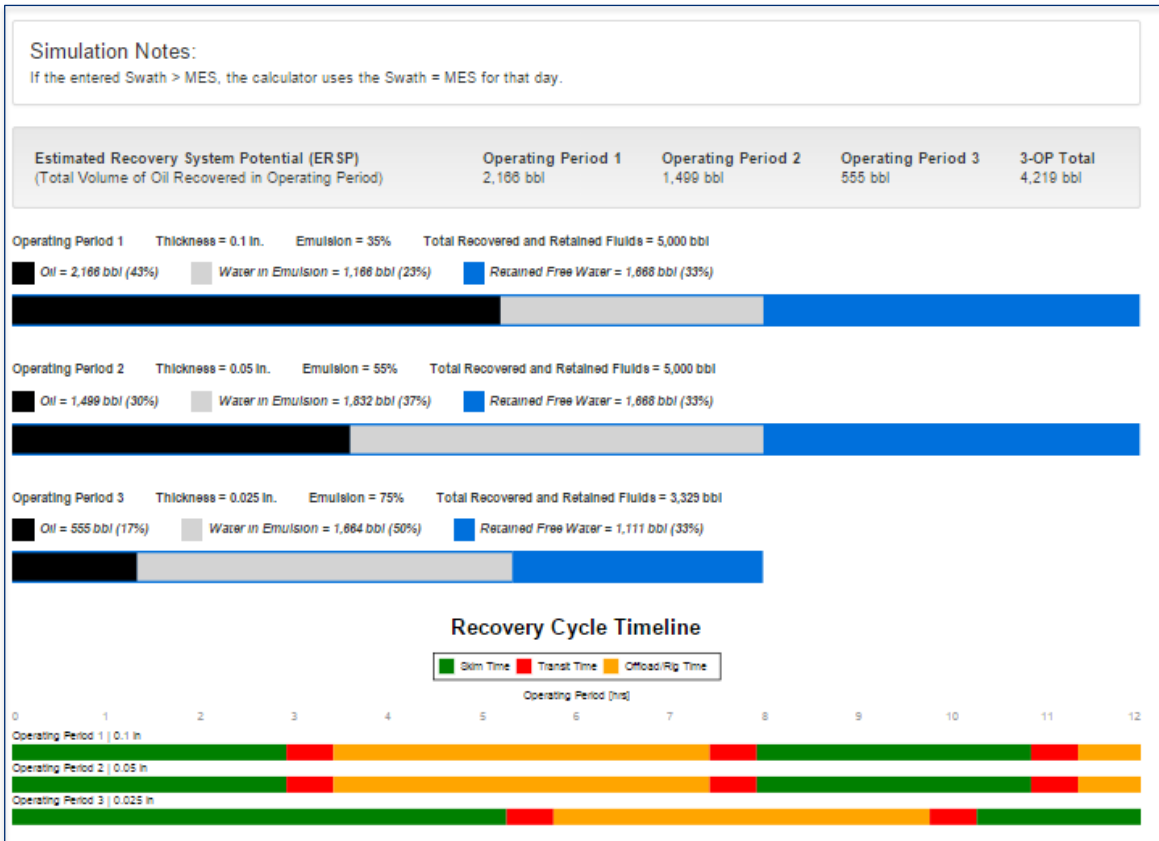
Figure 16. ERSP Graphical Outputs for Manatee Batch Spill
