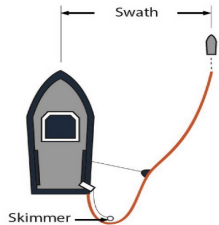
Figure 11. OSRV - J-boom
