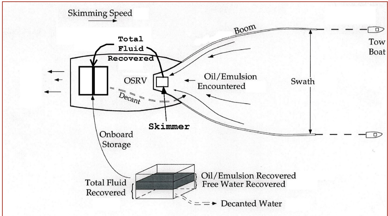
Figure 1. Advancing Skimming Recovery System Components.
